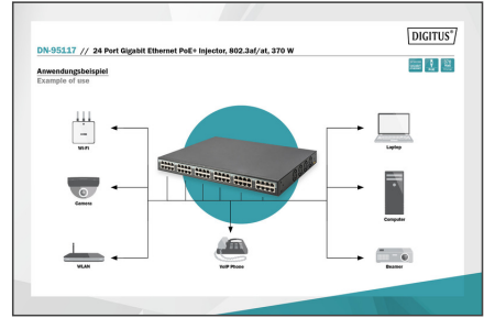
24 Port Gigabit Ethernet PoE + Injector, 802.3af/at, 370 W
