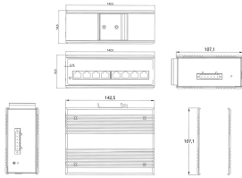
DN-ES8100 Industrial 8-Port Ethernet Switch, Unmanaged DIGITUS
