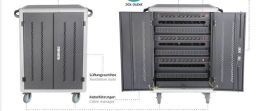
Anschlüsse/Connections
