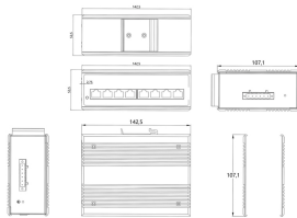
DN-688106 Industrial 8-Port Fast Ethernet Switch, Unmanaged
