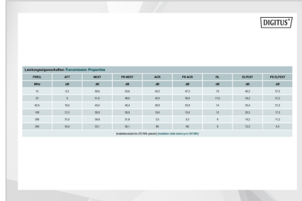
ASSNET250 CAT 6 U/UTP Installation Cable, 305 m, Eca
